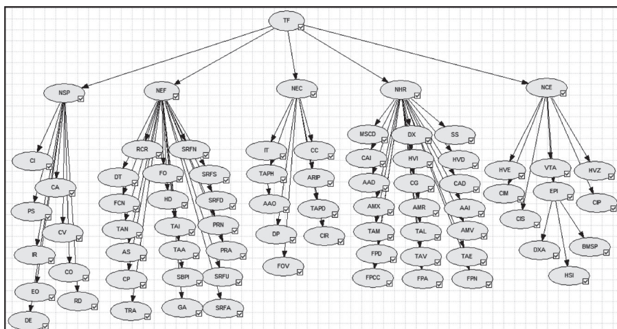
Figura 2. Red Bayesiana
